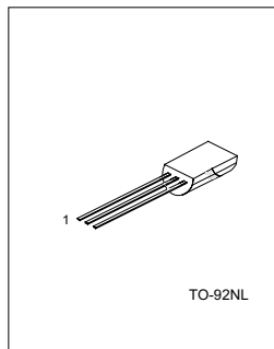
1: EMITTER 2: COLLECTOR 3: BASE
